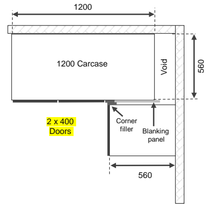
1200mm Corner base With 2 x 400mmW Door
