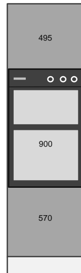
Medium 2120mmH Double Oven
