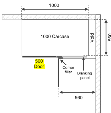
1000mm Corner base With 500mmW Door
