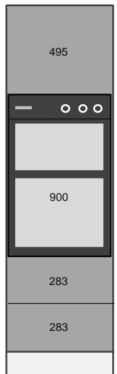
Medium 2120mmH Double Oven 2 x Deep Drawers
