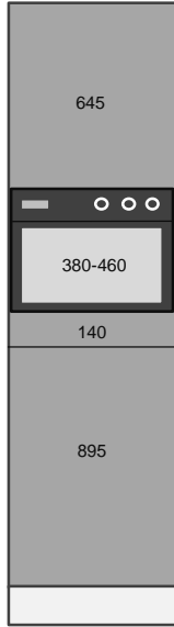
Taller 2300mmH Microwave
