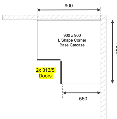
900mm x 900mm L Shape Corner base With 2 x 313/5mmW Doors
