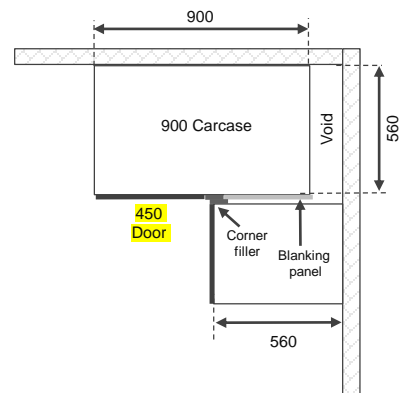
900mm Corner base With 450mmW Door
