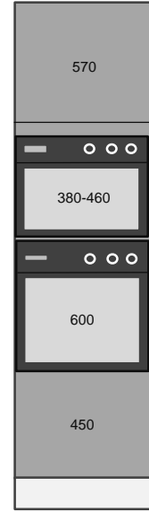
Taller 2300mmH Single Oven + Micro
