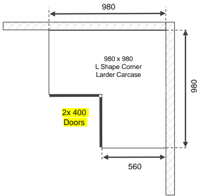
980mm x 980mm L Shape Corner Larder With 2 x 400mmW Doors
