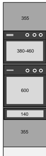
Medium 2120mmH Single Oven + Micro + Warming Drawer 1 x Deep Drawer
