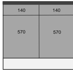
Drawerline - Double Bases Widths (mm) 800 900 1000 1200
