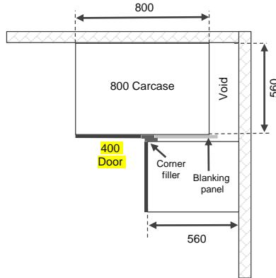
800mm Corner base With 400mmW Door
