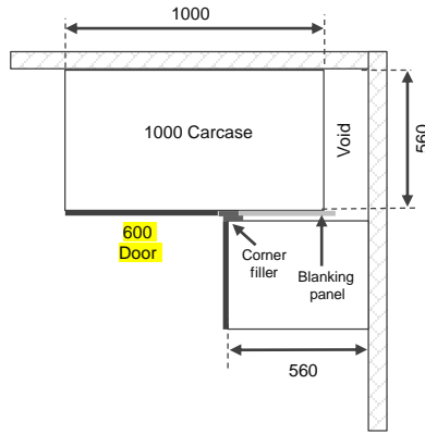
1000mm Corner base With 600mmW Door
