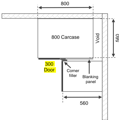
800mm Corner base With 300mmW Door
