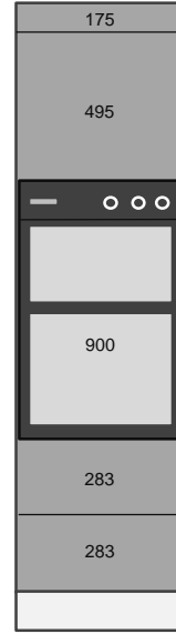
Taller 2300mmH Double Oven 2 x Deep Drawers
