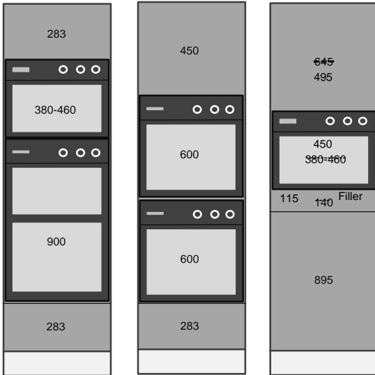
Medium 2120mmH Double Oven + Micro 1 x Deep Drawer
