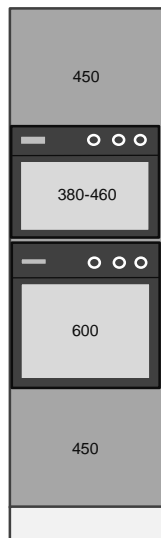
Medium 2120mmH Single Oven + Micro
