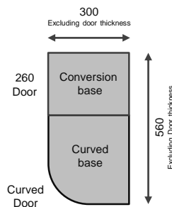
Curved base & 260mmW Conversion base
